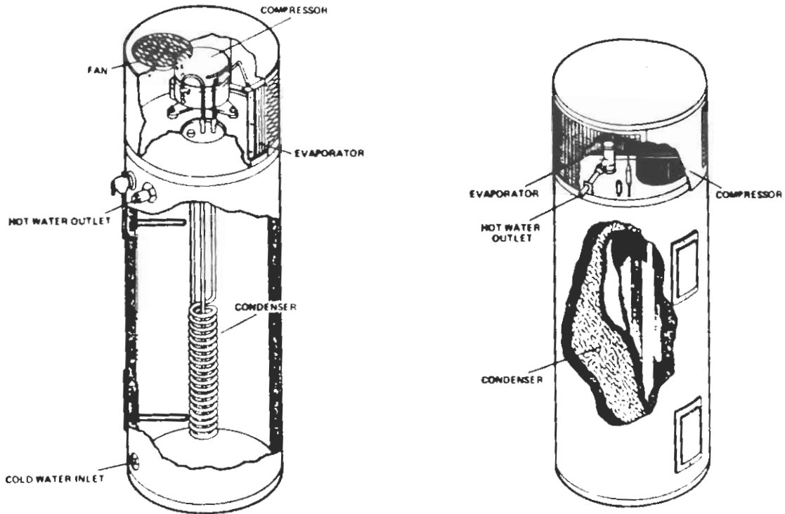
Figure 14-1. Integral HPWHs: Immersion (left) and External (right)
