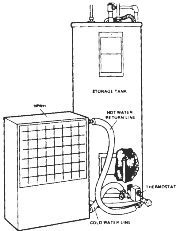
Figure 14-2. Remote HPWH
