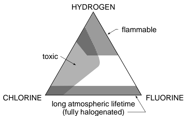
Figure 2. Trade-offs in flammability, toxicity, and atmospheric lifetime with changes in molecular chlorine, fluorine, and hydrogen content (from M. O. McLinden and D. A. Didion, 1987 8 )
