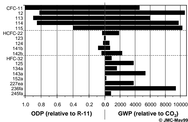
Figure 4. Ozone depletion potential (ODP) contrasted to global warming potential (GWP) for key single-compound refrigerants (based on data from reference 14): CFCs generally have high ODP and GWP. HCFCs generally have much lower ODP and GWP. HFCs offer near-zero ODP, but some have comparatively high GWPs.
