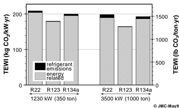
Figure 5. Greenhouse gas emissions (expressed as equivalent carbon dioxide) per unit of cooling per year—TEWI—for the best available chillers in two representative capacities
